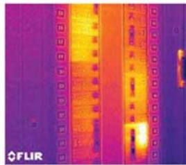
Breaker Panel
