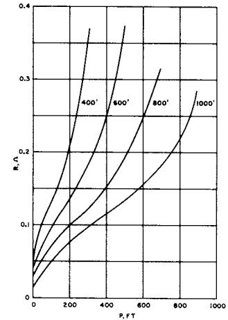
Fig. 29: Earth resistance curves for a substation
